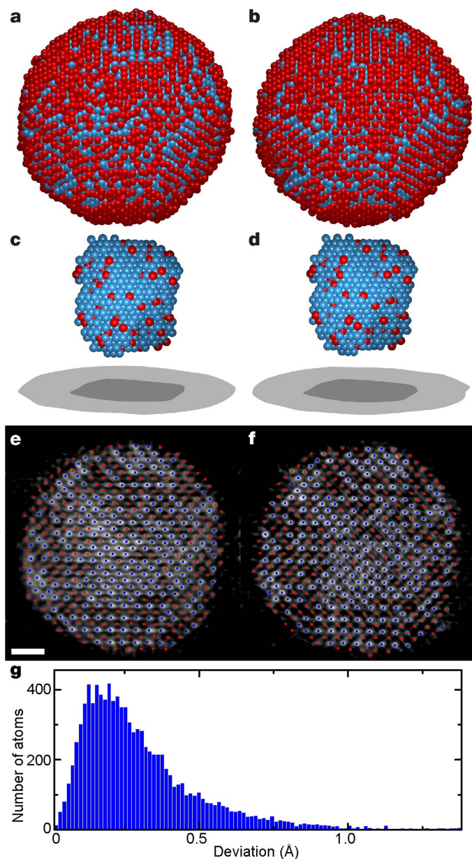
Extended Data Fig. 1 | Consistency check of the AET measurements. a, b, 3D atomic models (Pt in blue and Fe in red) of particle 1, obtained from two independent experimental measurements. c, d, Pt-rich cores cropped from the atomic models shown in a and b , respectively. e, f, The same atomic layer of the nanoparticle along the [010] direction (Pt in blue and Fe in red), obtained from the two independent measurements. Scale bar, 1 nm. g, Histogram of the deviation of the common atoms between the two independent measurements. By dividing the common atoms by the average number of atoms in the two measurements, we estimated that 95.4% of the atoms are consistent. The average deviation between the two independent measurements is 37 pm. According to the statistical analysis of error propagation, the precision of the AET measurement is 37 \text{ pm} / \sqrt{2} = 26 \text{ pm} . (See Methods for details.).
