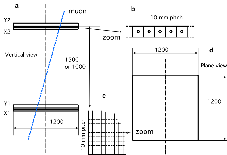
Extended Data Figure 3 | Overview of the scintillator hodoscopes (KEK). a , Vertical view of the detector, consisting of two units of orthogonal double scintillator layers. A blue arrow indicates a muon track passing through the whole instrument. b , Cross-section of a scintillator
