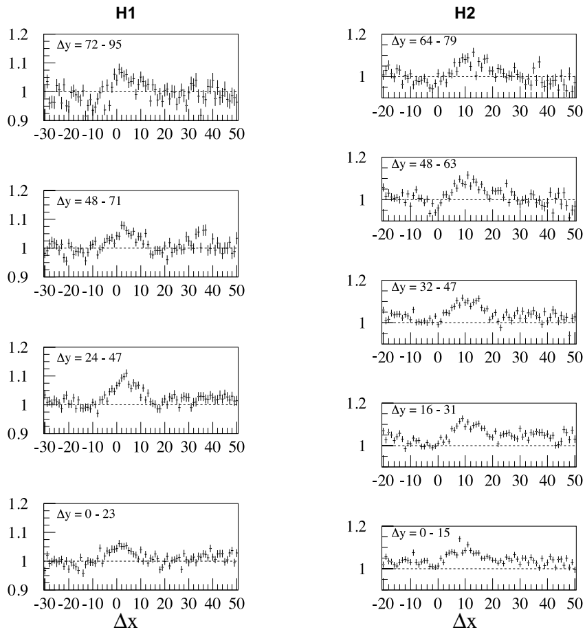
Extended Data Figure 4 | Slices of the data for the scintillator hodoscopes. Left, relative yield of the measurement to the simulation (including known structures) at position H1 for four slices (the width of each bin is 24 \Delta y ). Right, relative yield at position H2 for five slices (the width of each bin is 16 \Delta y ). Error bars show statistical errors of 1\sigma (standard deviation).
