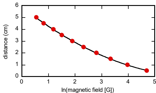
Figure 3: Calibration of the magnetic field of a Nd-FeB magnet with distance. The calibration is more precise when performed in function of the logarithm of the magnetic field (in gauss here), since the value of the field varies over two decades with distance. In this experiment, a second order polynomial fit is sufficient to describe the calibration points.
