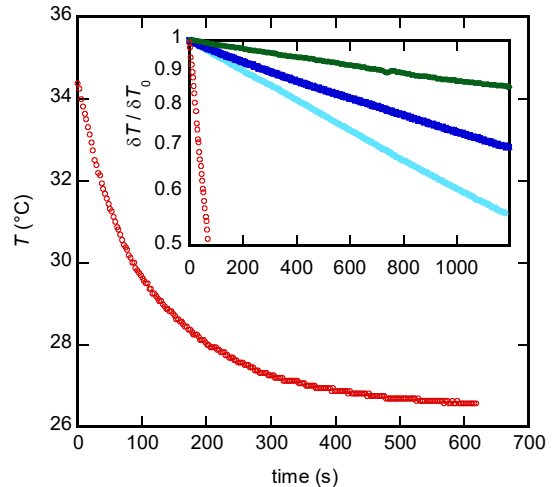
Figure 5: Exponential decay of the temperature of 16 cL of water in a plastic goblet initially heated at 34 °C and put in a room at 25 °C. Inset: renormalized temperature (T - T_{rt})/(T_i - T_{rt}) in a log scale, as a function of time, for different configurations; from left to right, a goblet immersed in a large volume of water at room temperature (also represented in the main frame of the figure), a goblet in air, a goblet in air with wool cover on its sides and below, a goblet fully protected by wool. The corresponding heat loss are respectively 5 \text{ W K}^{-1} ( \tau = 130 \text{ s} ), 0.34 \text{ W K}^{-1} ( \tau = 2000 \text{ s} ), 0.2 \text{ W K}^{-1} ( \tau = 3300 \text{ s} ), and 0.09 \text{ W K}^{-1} ( \tau = 7700 \text{ s} ).
